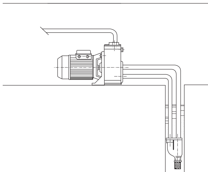
Fig. 14 Installation principle for JDBasic
