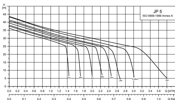
Fig. 8 Performance curves for JP 5 and JP 6
