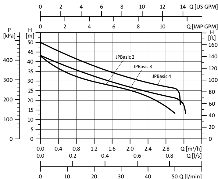
Fig. 25 Performance curves for JPBASIC
