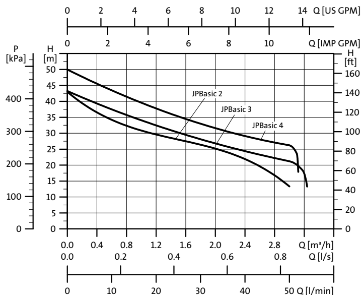
Fig. 31 Performance curves for JPBASIC PT
