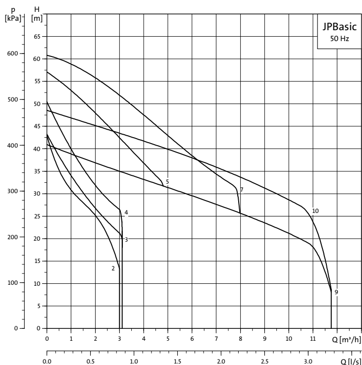
Fig. 12 Performance curves for JPBASIC
