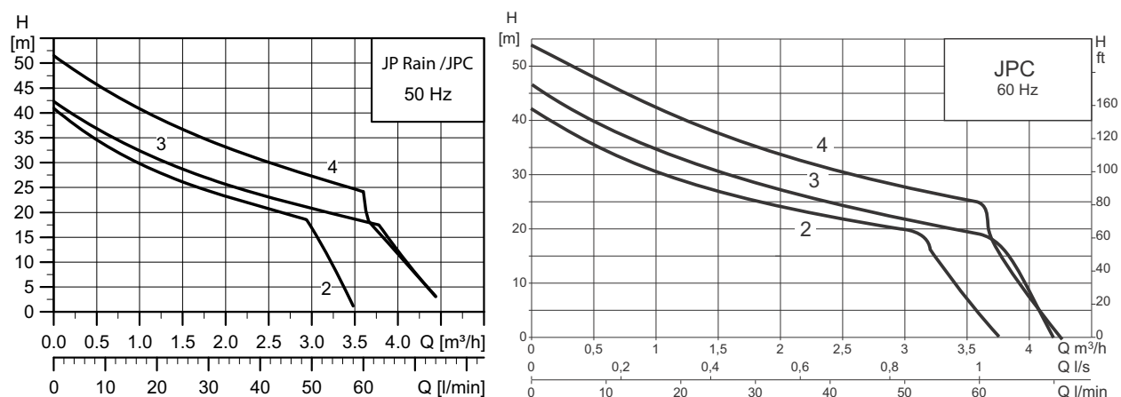
Fig. 10 Performance curves for JPC/JPRain 2, JPC/JPRain 3 and JPC/JPRain 4
