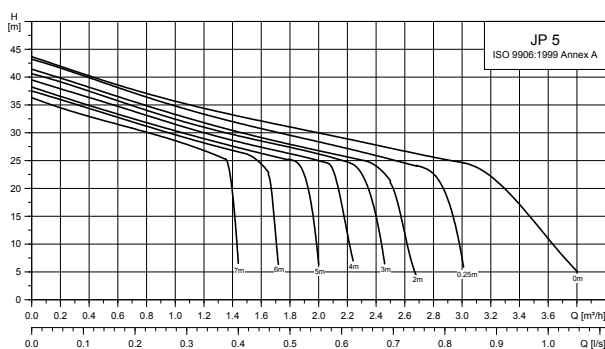
Fig. 17 Performance curves for JP 5 and JP 6
