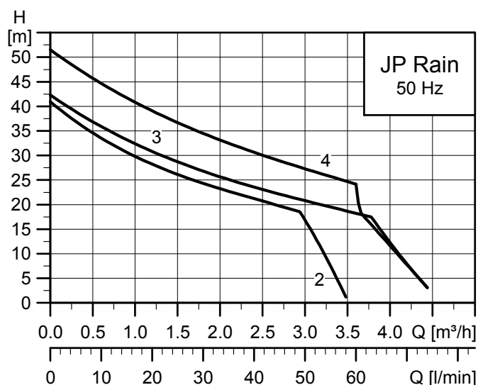
Fig. 23 Performance curves for JPRain 2, JPRain 3 and JPRain 4
