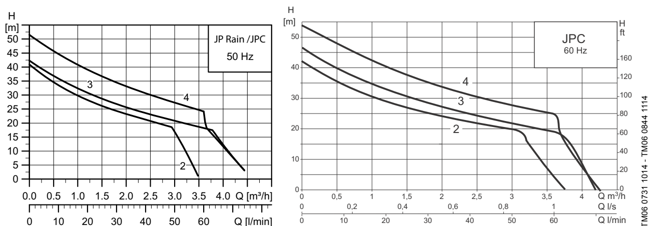
Fig. 29 Performance curves for JPC/JPRain 2, JPC/JPRain 3 and JPC/JPRain 4
